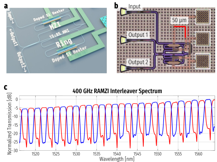
Figure 3. (a) Design rendering of a RAMZI with a 400 GHz FSR. (b) Microscope image of the fabricated device. (c) Measured transmission spectra of the interleaver. The red and blue curves correspond to the two output ports.
