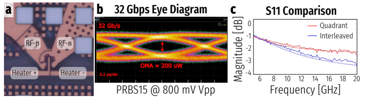
Figure 9. (a) Microscope image of a fabricated interleaved contact microdisk modulator. (b) Open eye diagram at 32 Gbps with PRBS15 driven by 800 mV peak-to-peak voltage. (c) Measured S11 frequency response after de-embedding the pads and connected metal traces, showing reduced back reflections due to better impedance matching with greater number of parallel interleaved contacts [56].
