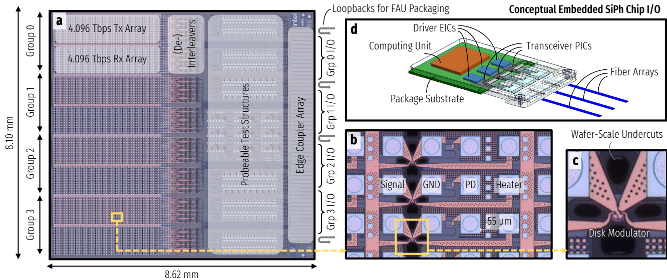
Figure 2. Microscope images of the designed and fabricated transceiver PIC, where each (a) 8.10 mm×8.62 mm chip consists of four groups of Tx/Rx arrays targeting 4.096 Tbps/group, probable test structures of link subcomponents for pre-packaging characterization of process variations and screening of KGDs, and custom suspended edge couplers [12] providing low-loss optical I/O. Each 4.096 Tbps transceiver group consists of four 1.024 Tbps links with the architecture of Fig. 1a. The Tx/Rx arrays feature (b) electrical pads at a 55 μm pitch for EIC flip-chip bonding and (c) wafer-scale substrate undercuts for improving the thermal tuning efficiency of and reducing the thermal crosstalk between the thermal phase shifters. (d) A conceptual chip I/O configuration shows multiple transceiver PICs embedded onto a single platform, next to the computing socket.
