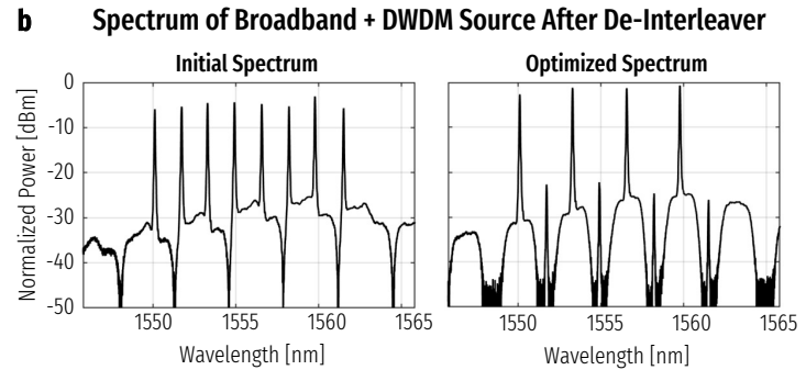
Figure 5. (a) Experimental setup for the interleaver auto-tuning process, where PC: polarization controller, OPM: optical power meter, PS: power supply, and DUT: device under test. (b) RAMZI interleaver spectra with DWDM source before and after the auto-tuning, showing an optimized extinction ratio of over 20 dB and the precise alignment of the pass-bands to the DWDM channels after tuning [55].
